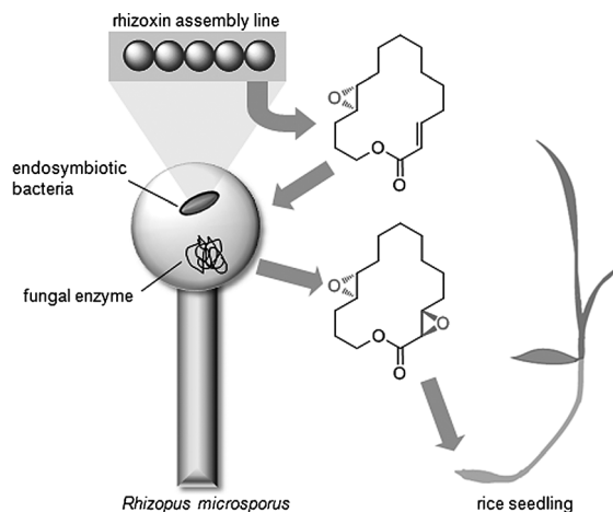
Figure 5. Flowchart of synergistic phytotoxin production. The bacterial endosymbiont produces the rhizoxin backbone, which is tailored by an oxygenase provided by the fungal host to render it more effective against rice seedlings.
